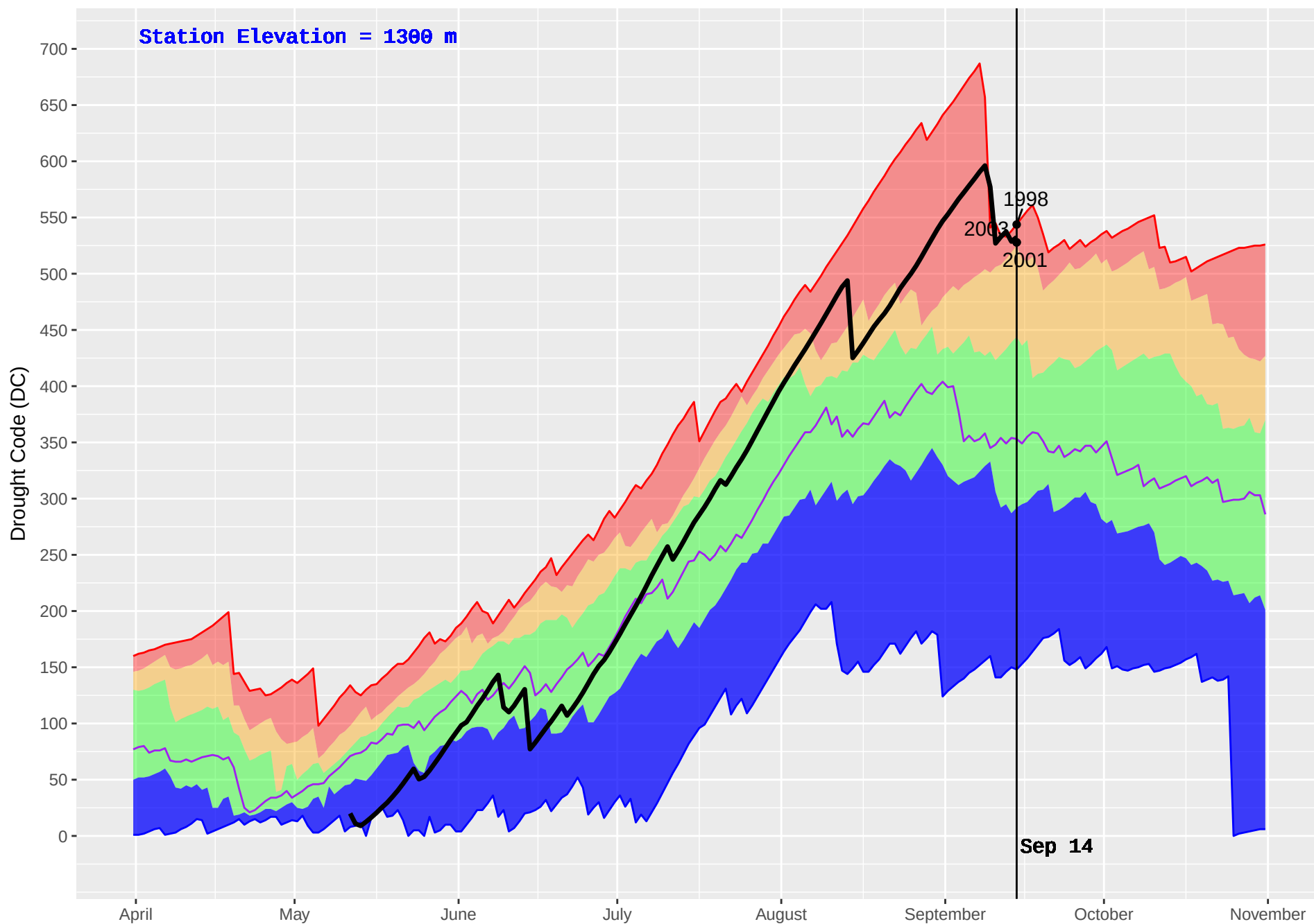
MARION (367) : Historical (1994–2016) and Current (2017) Noon Drought Code (DC)
